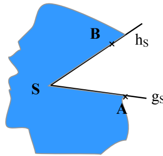
Winkel \angle h_s, g_s Winkel \angle BSA
